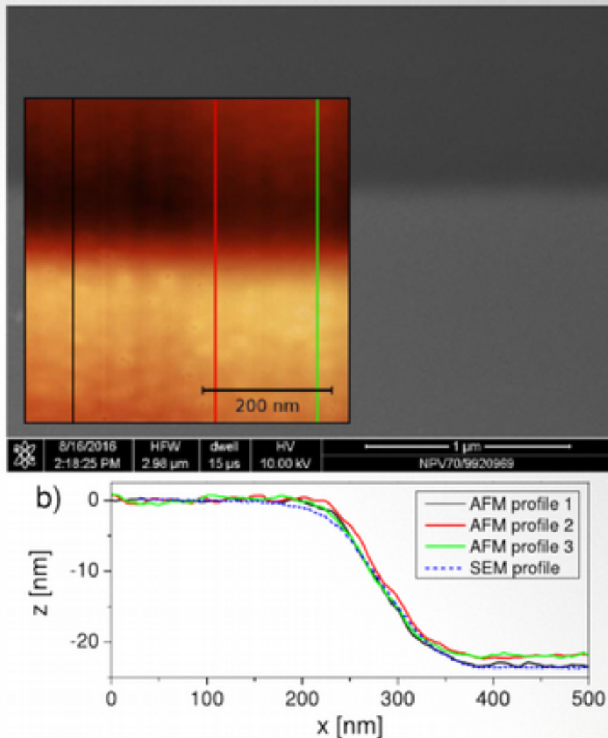
Fig. 2. a) Scanning electron microscopy image of the edge of a single wire of the Pt (15 nm)/[Co(0.6 nm)/Pt(1.5 nm)] 4 ML. Bright area is the wire's surface and dark area is the Si substrate. Inset shows the AFM image of the analogous wire's edge for comparison. Non-coated, silicon AFM probe in soft tapping mode was used having dimensions of 150 × 30 × 2.7 μm with a tip height of 17 μm and a tip radius below 10 nm. Color lines represent profiles shown below. b) Profiles extracted from the AFM and SEM images, confirming the edge taper visible on the images above. The z-coordinate for the SEM profile corresponds to the change of image brightness. It was scaled and superimposed on the AFM profiles. Lines' colors correspond to the profile markings on the AFM and SEM images. (For interpretation of the references to colour in this figure legend, the reader is referred to the web version of this article.)
