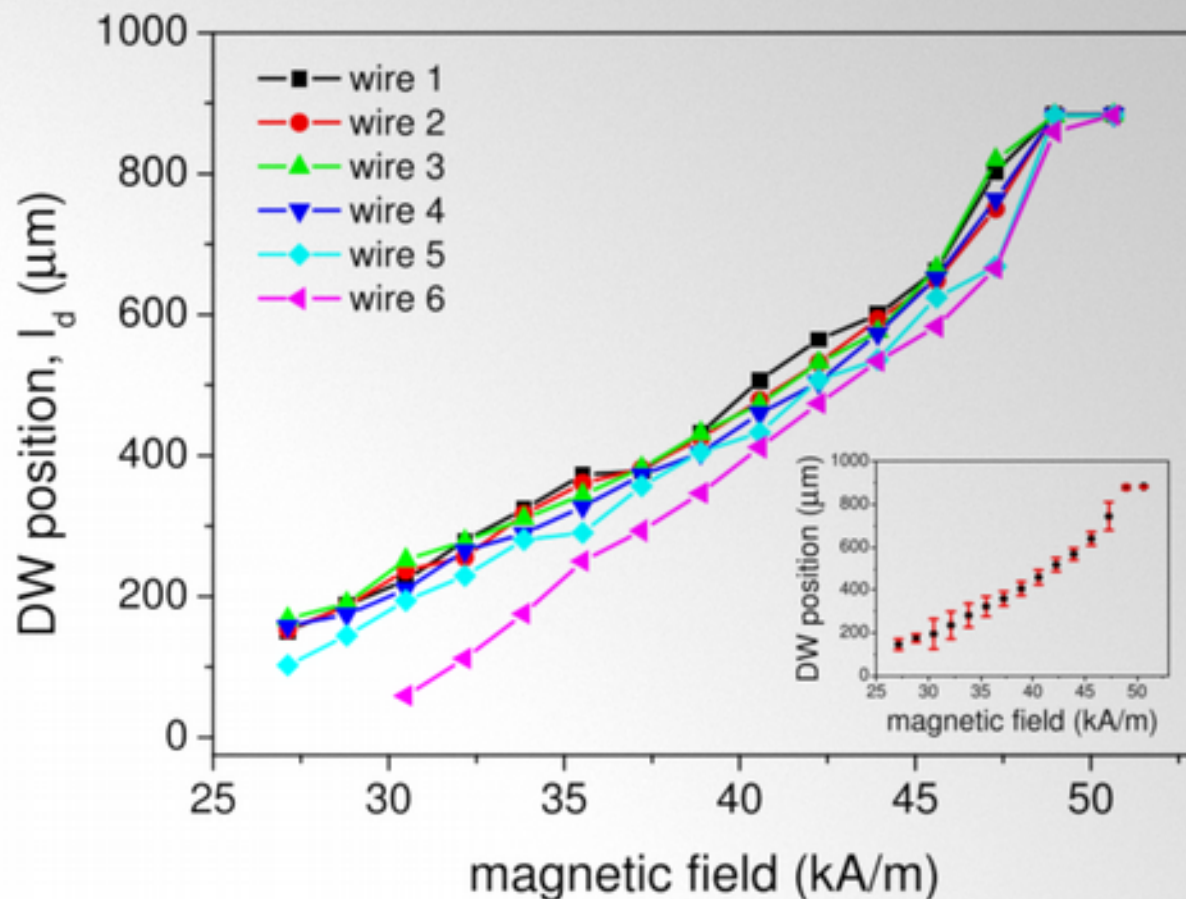
Fig. 5. Experimentally determined DW positions as functions of magnetic field (see Section 2) for wires of 10\text{ }\mu\text{m} widths. The wires are numbered according to their order in Fig. 4 from top to bottom. The inset presents an average DW position determined from the behavior of all six wires (black line) with one standard deviation (red error bars) as a function of magnetic field. (For interpretation of the references to colour in this figure legend, the reader is referred to the web version of this article.)
