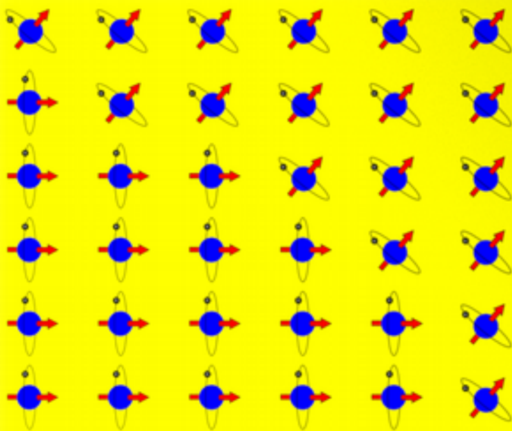
atomistic description
