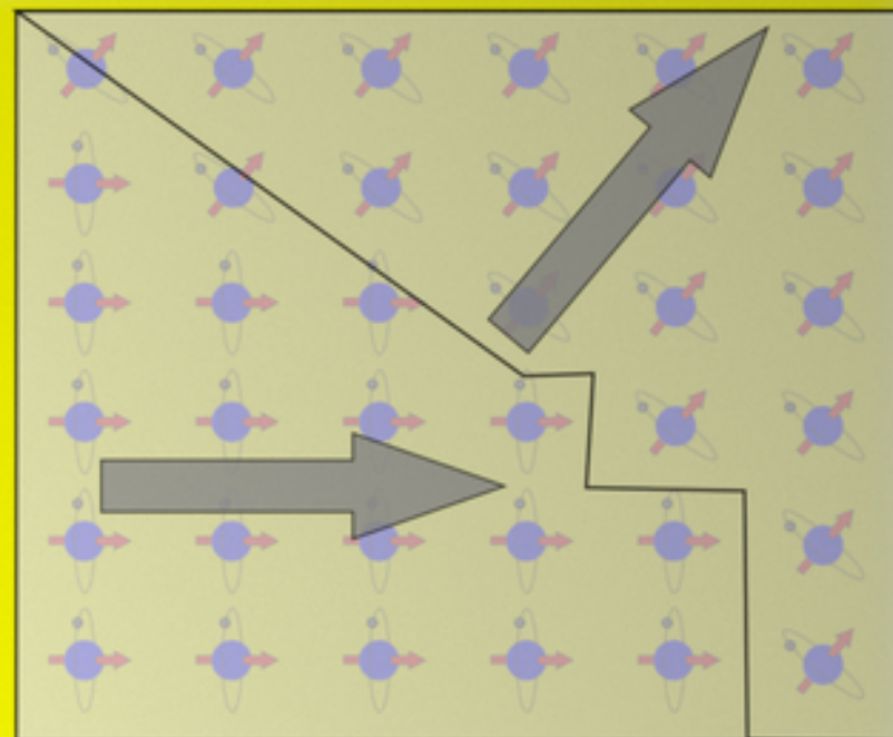
micromagnetic description
