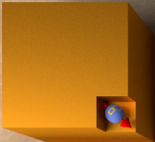
atomistic description
